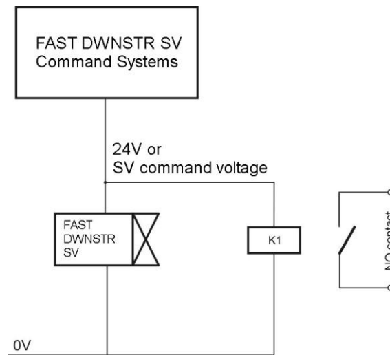
Figure 13.10 Example of generation of high-speed closing signal
