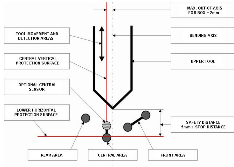
Fig. 13.3 Positioning with respect to the axis of the tool
