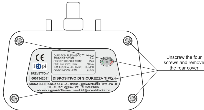
Fig.18.1 Removal of the rear cover
