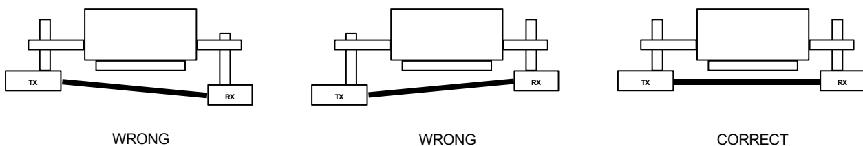
Fig. 13.5 Adjustment longitudinal with respect to the bending line
