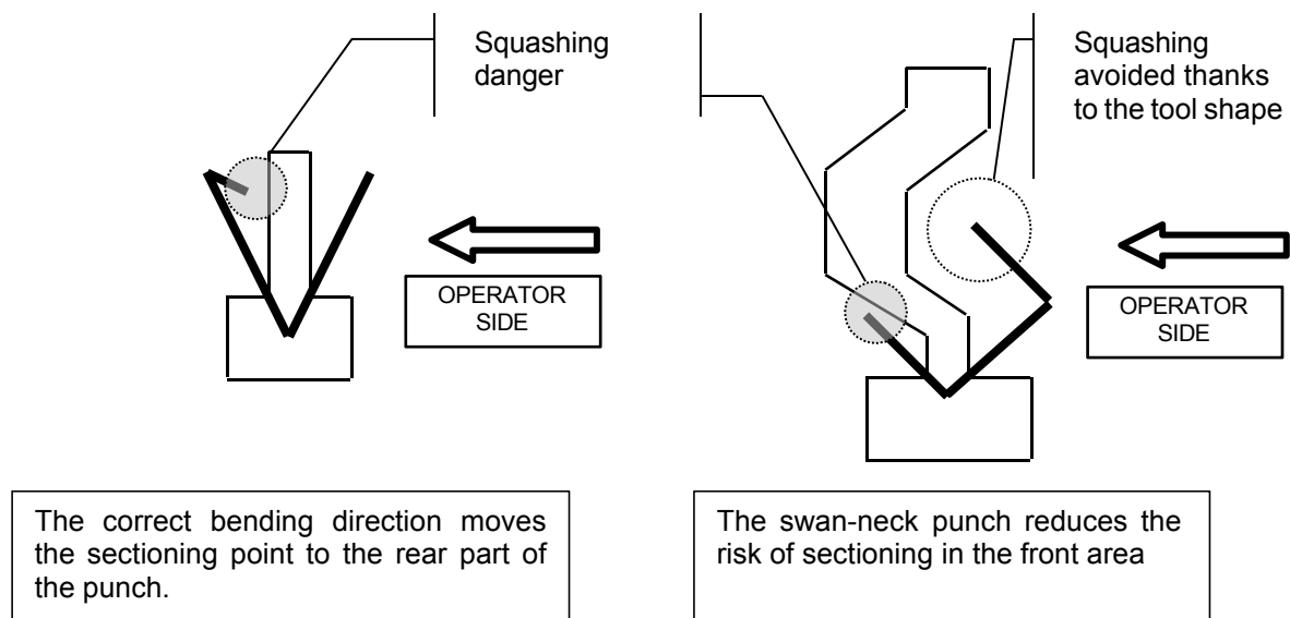
Fig. 11.3 Reduction of the residual risks
