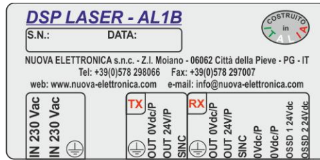
Fig. 12.8 Identification plate of AL1B module
